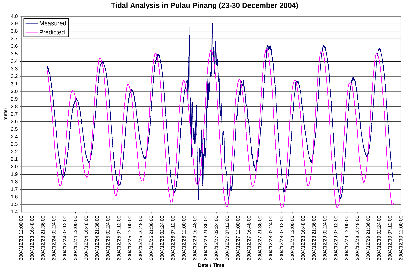
Figure 4: Tidal records from Penang indicating sea levels during the tsunami (Dept. of Survey & Mapping Malaysia)
