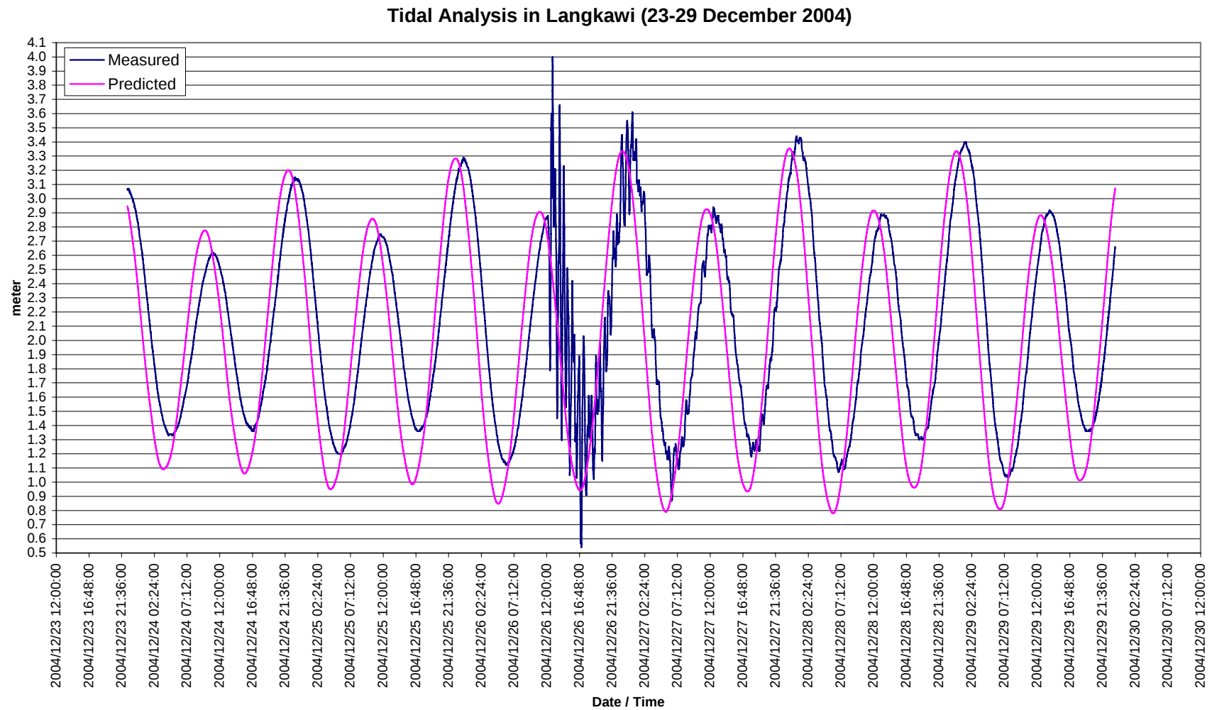
Figure 3: Tidal records from Langkawi indicating sea levels during the tsunami (Dept. of Survey & Mapping Malaysia)
